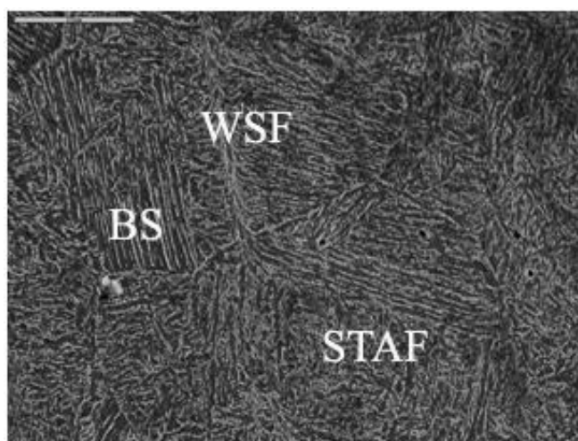
Figure 6. SEM image Microstructure after completed isothermal decomposition at 450°C – bar 50µm.
